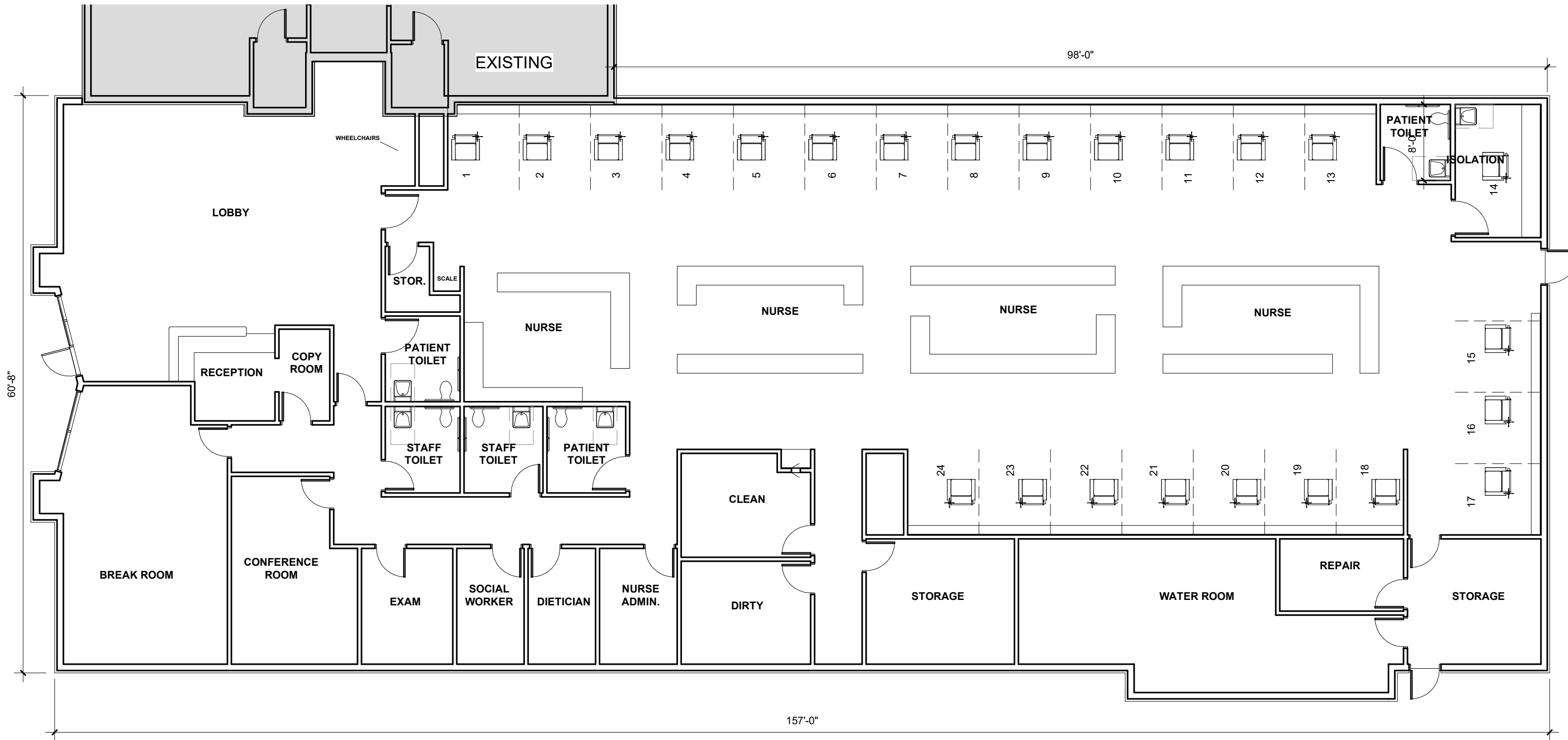
1 Floor Plan 1" = 10'-0"
